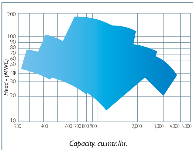
Horizontal Split Case Pump "LN" Series Coverage Chart 4 Pole 50Hz
