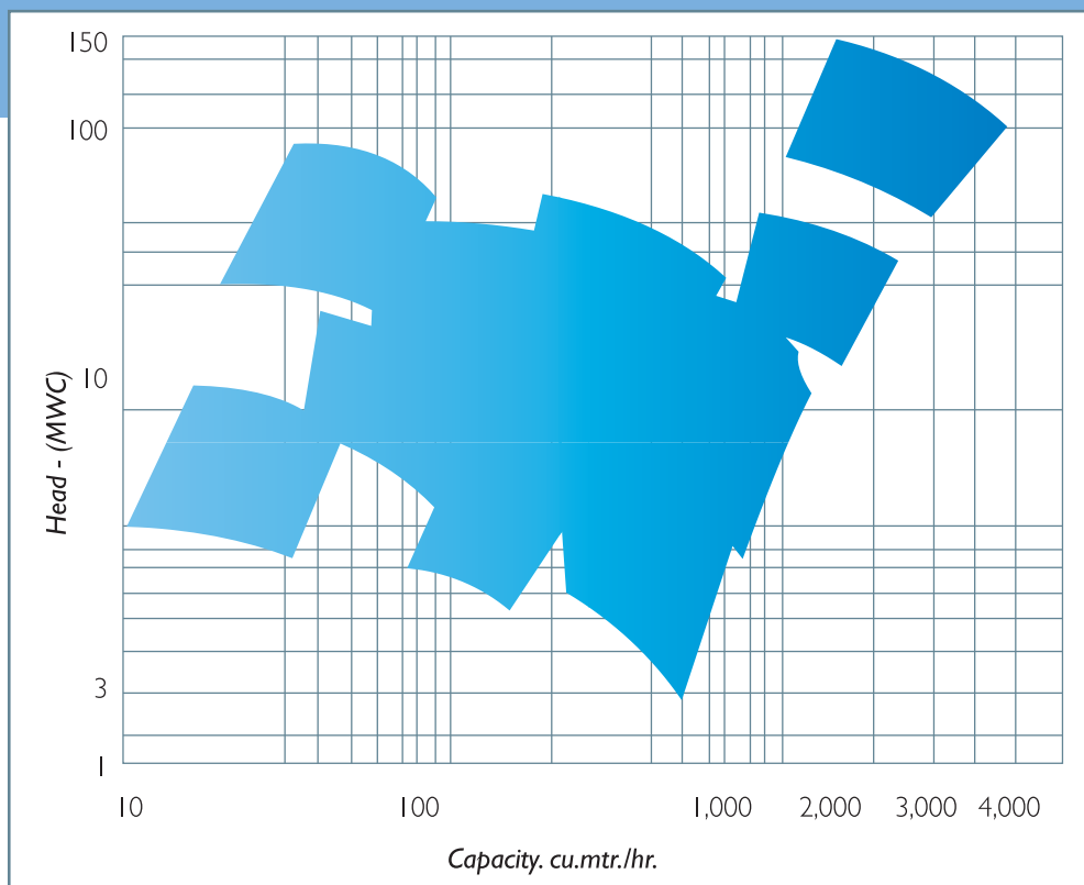
Horizontal Split Case Pump "LR" Series Coverage Chart
