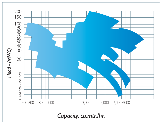
Horizontal Split Case Pump "LN" Series Coverage Chart 6, 8 & 10 Pole 50Hz
